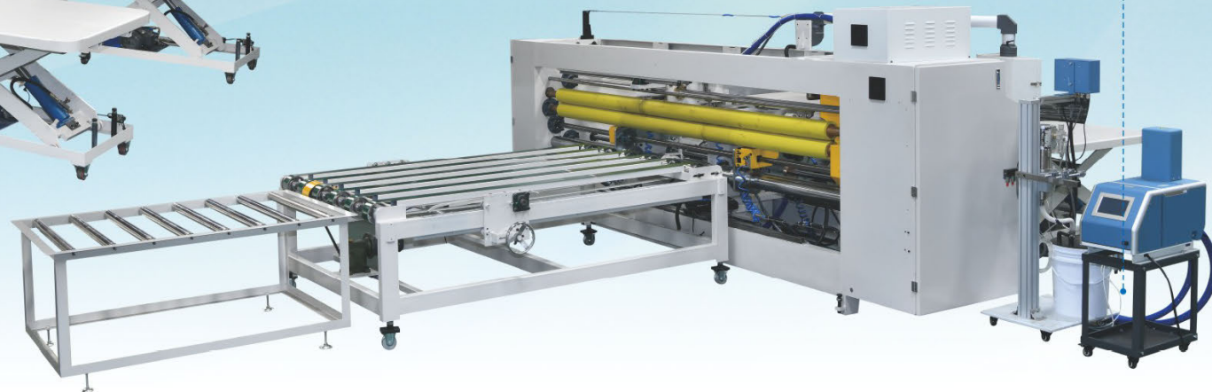
配备外置独立冷胶系统和热熔胶喷胶系统，自动喷胶 Equipped with external independent cold glue system and hot melt applicator, automatic glue spraying
